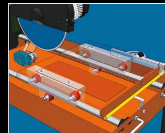
Working table with sliding carriage equipped with 6 adjustable nylon wheels and 12 ball-bearings to get a perfect precision, stability and sliding.
